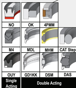
Piston Seals
