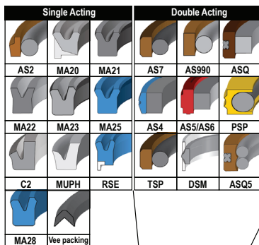
Piston Seals
