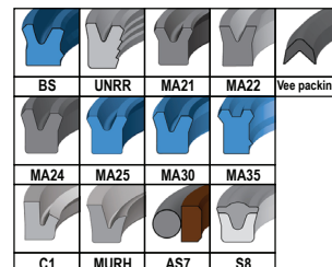
Rod Seals
