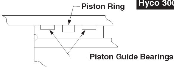
Double Acting
