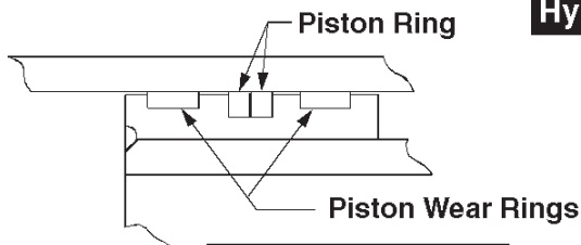
Double Acting
