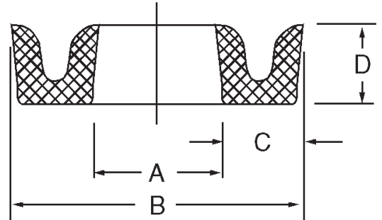
Contoured Profile (-1)
