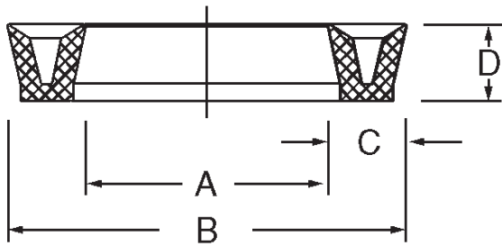
Rectangular Profile
